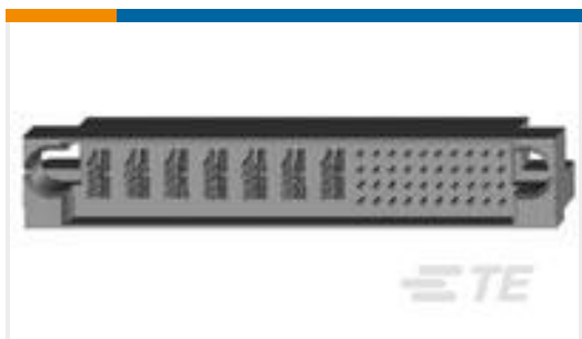
TE 零件编号6450122-8 MBXL R/A HDR 7P+40S
