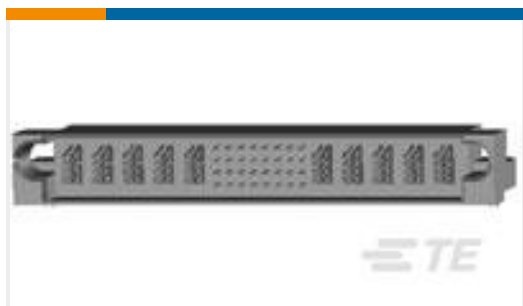
TE 零件编号2-6450120-4 MBXL R/A HDR 5P+32S+5P
